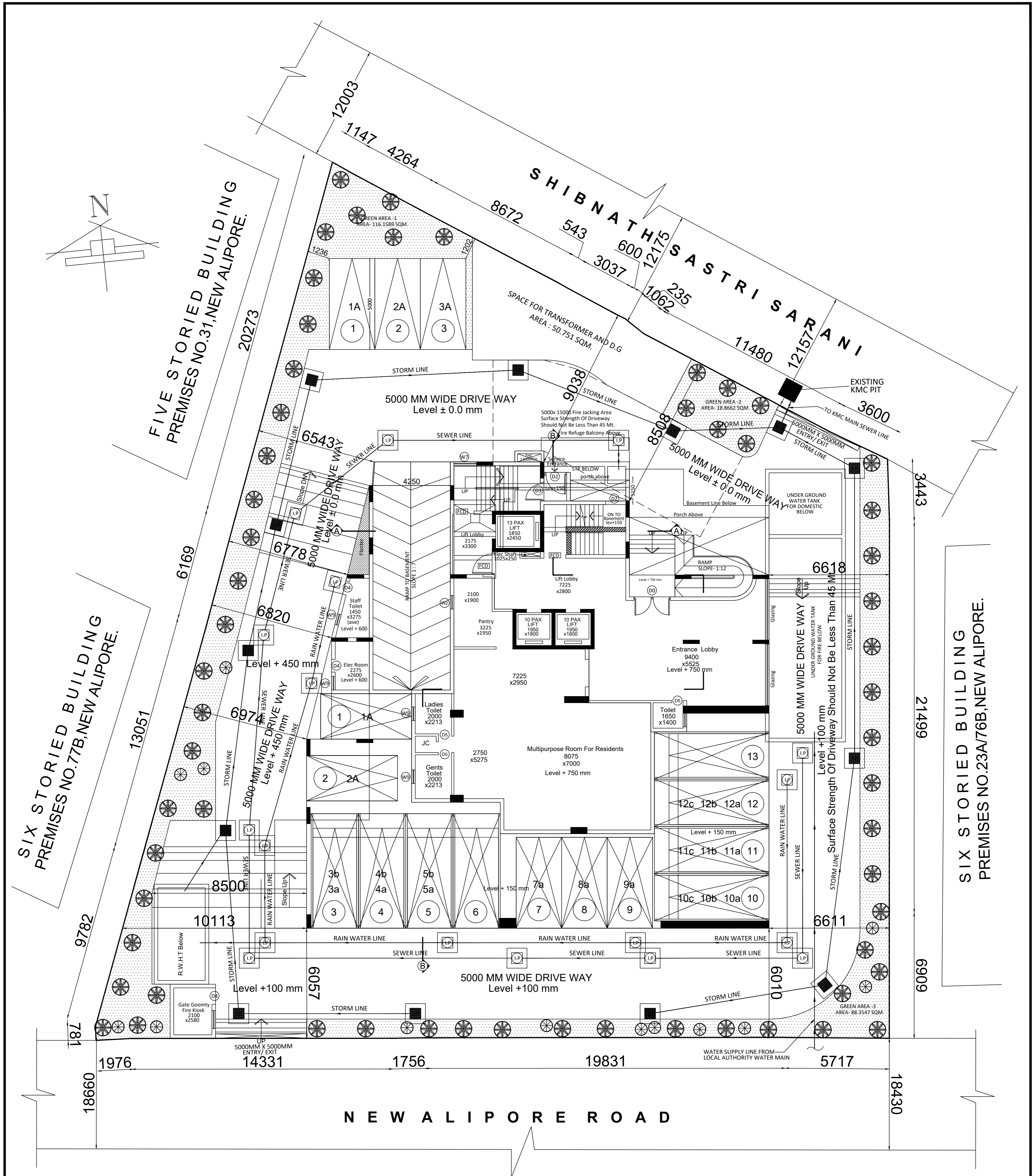
GROUND FLOOR PLAN SCALE- 1: 100
